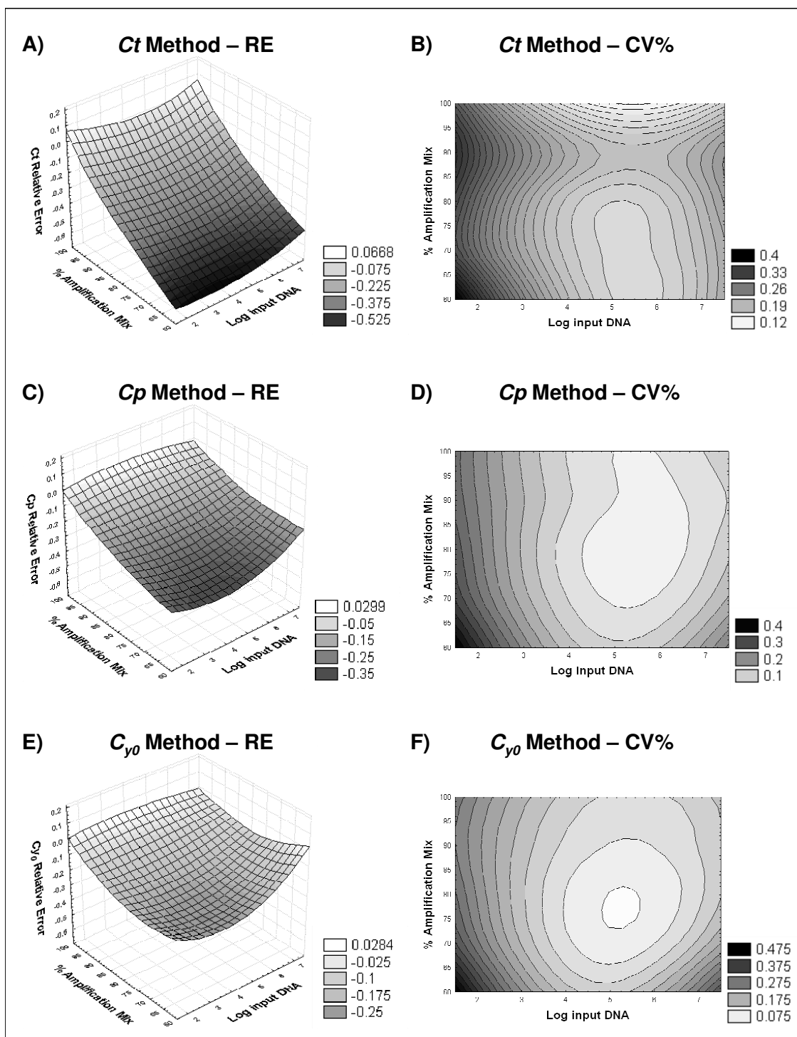
Figure 5 Comparison of the Ct, Cp and C_{y0} methods in terms of precision and accuracy. The accuracy of each method has been reported as Relative Error (RE = expected value – estimated value) while the precision was evaluated measuring the variation coefficient (CV%). The 3D plots show the variation of relative error in relation to amplification mix percentage and \log_{10} input DNA for the Ct (A), Cp (C) and C_{y0} (E) methods. The areas in the level curve graphs represent the CV% values obtained for each amplification mix percentage and \log_{10} input DNA combination using the Ct (B), Cp (D) and C_{y0} (F) methods.
