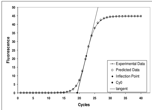
Figure 1 Example of modelling PCR amplification with a 5-parameter Richards function. Effectiveness of this model is illustrated by the predicted values generated by Eq. 3 (open circles) that agree with the observed fluorescence (dot and line). Curve-fitting of experimentally derived fluorescence dataset to Eq. 3 generates values for the kinetic parameters from which the inflection point (solid black rhombus) and the slope of the curve can be derived. The quantitative entity Cy_0 (solid black dot), used in the proposed method, shows the cross point between the x-axis and the tangent crossing the inflection point of real-time PCR fluorescence curve.
